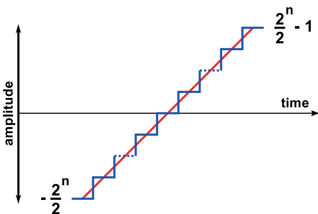
Quantisation including zero (mid-tread)
